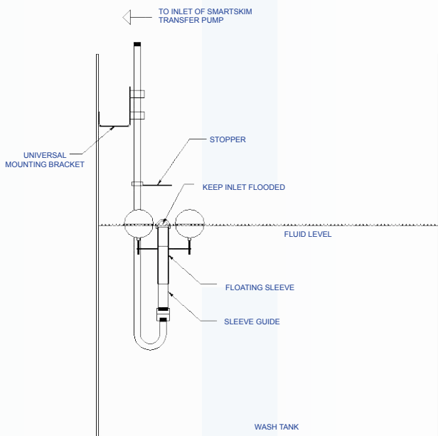
Typical 7" Skimmer Setup
